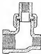
Fig. 3155. CARBURETOR UNION-TEE.
